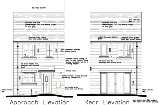
Approach Elevation
