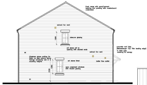
Gable Elevation (plot 11)
