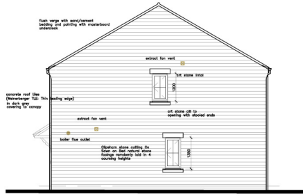
Gable Elevation (plot 12)
